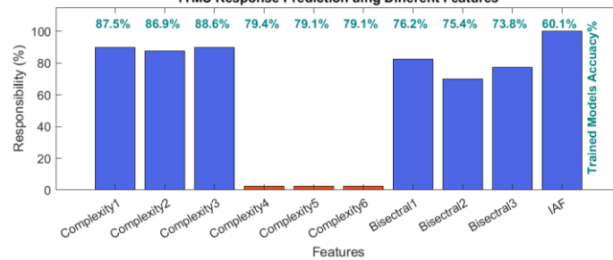
rTMS Response Prediction using Different Features
